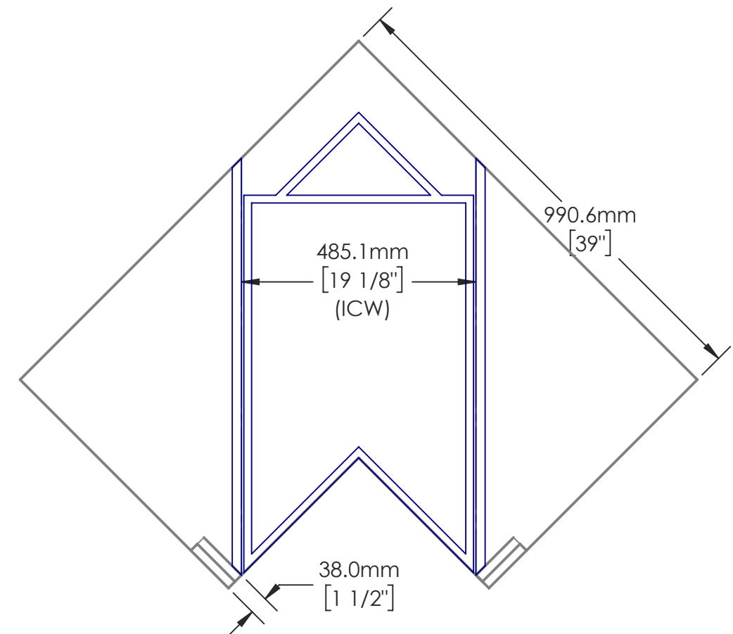
39" CABINET SIZE REFERENCE DRAWING
