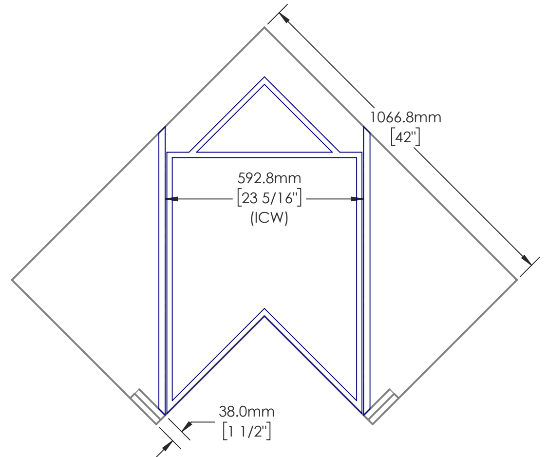
42" CABINET SIZE REFERENCE DRAWING
